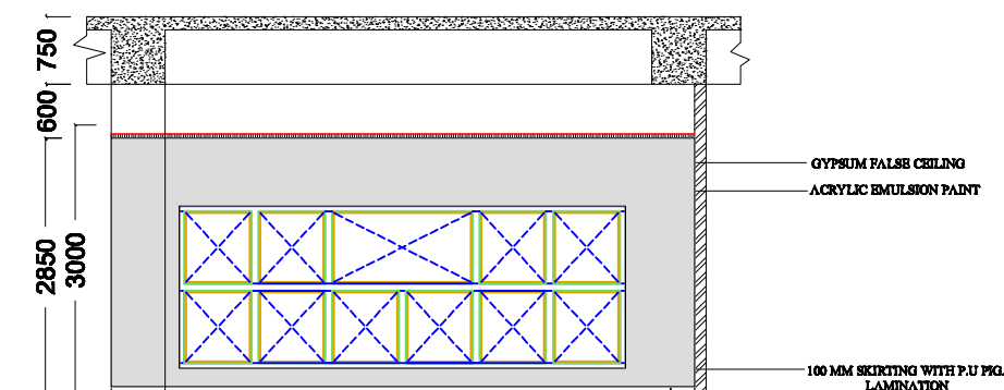
ELEVATION D
