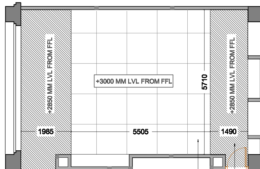
REFLECTED CEILING PLAN LAYOUT
