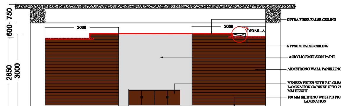
ELEVATION AT A
